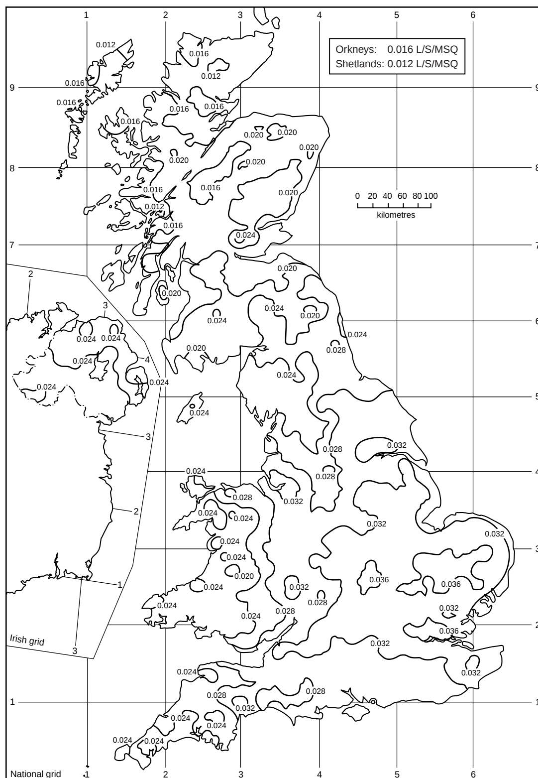
Figure NB.2 — Rainfall intensity, r , for a 2 min duration storm event with return period of 5 years (in l/s per m²)
