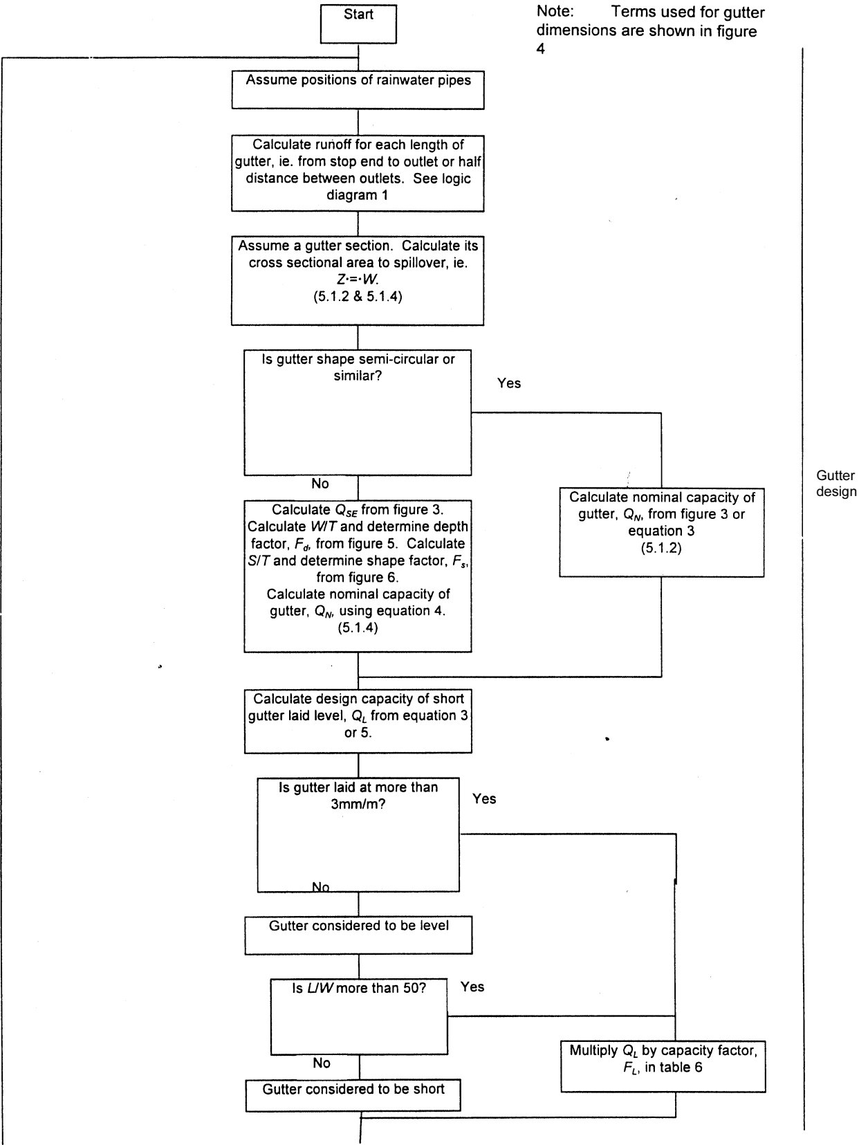
Logic diagram 4 — Eaves gutters
